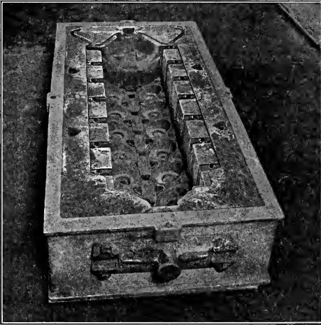
Fig. 61. Drag Half of Mould Ready for Setting the Cores.
